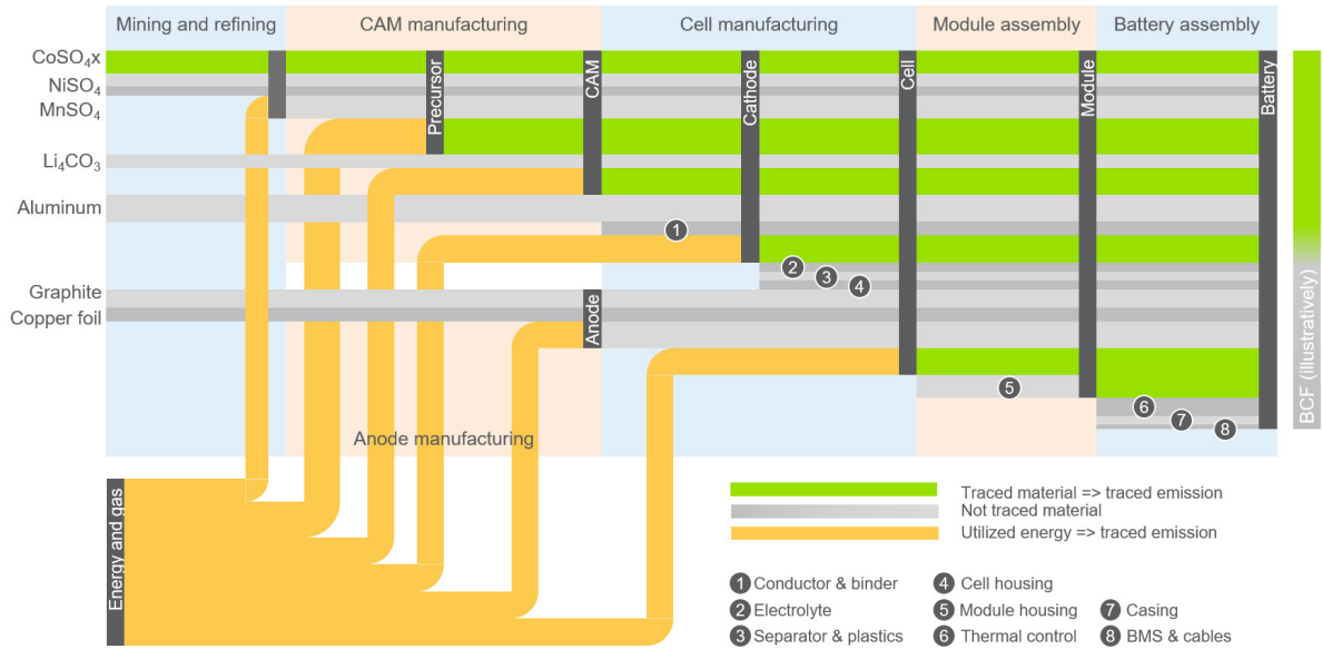
Figure 1. Illustrative process of GHG aggregation for NMC811 type of battery
